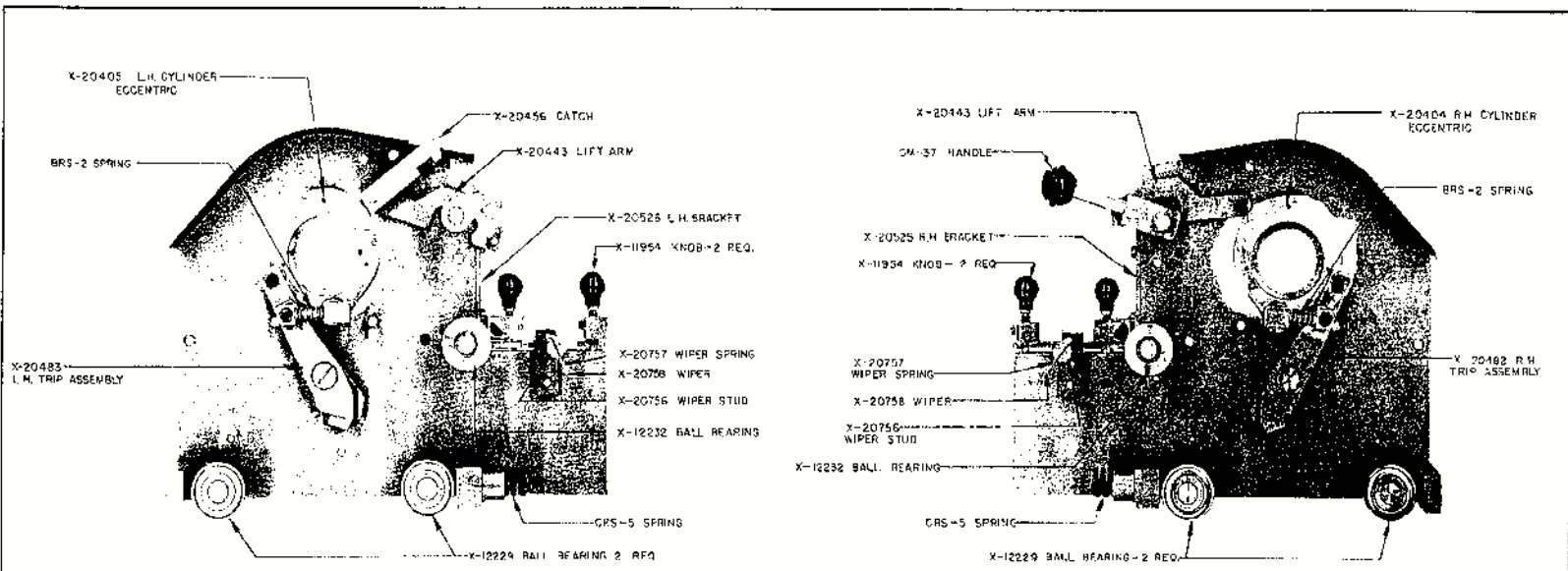
INSIDE VIEW OF CARRIAGE SIDE PLATE—LEFT SIDE
