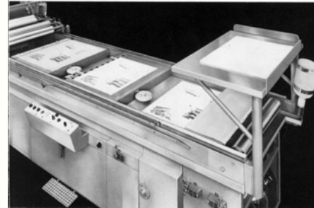
Convenient stock table and delivery tray—adjustable speed water supply drum with Baldwin water level system.
