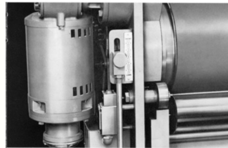
Adjustment for printing short or long.
