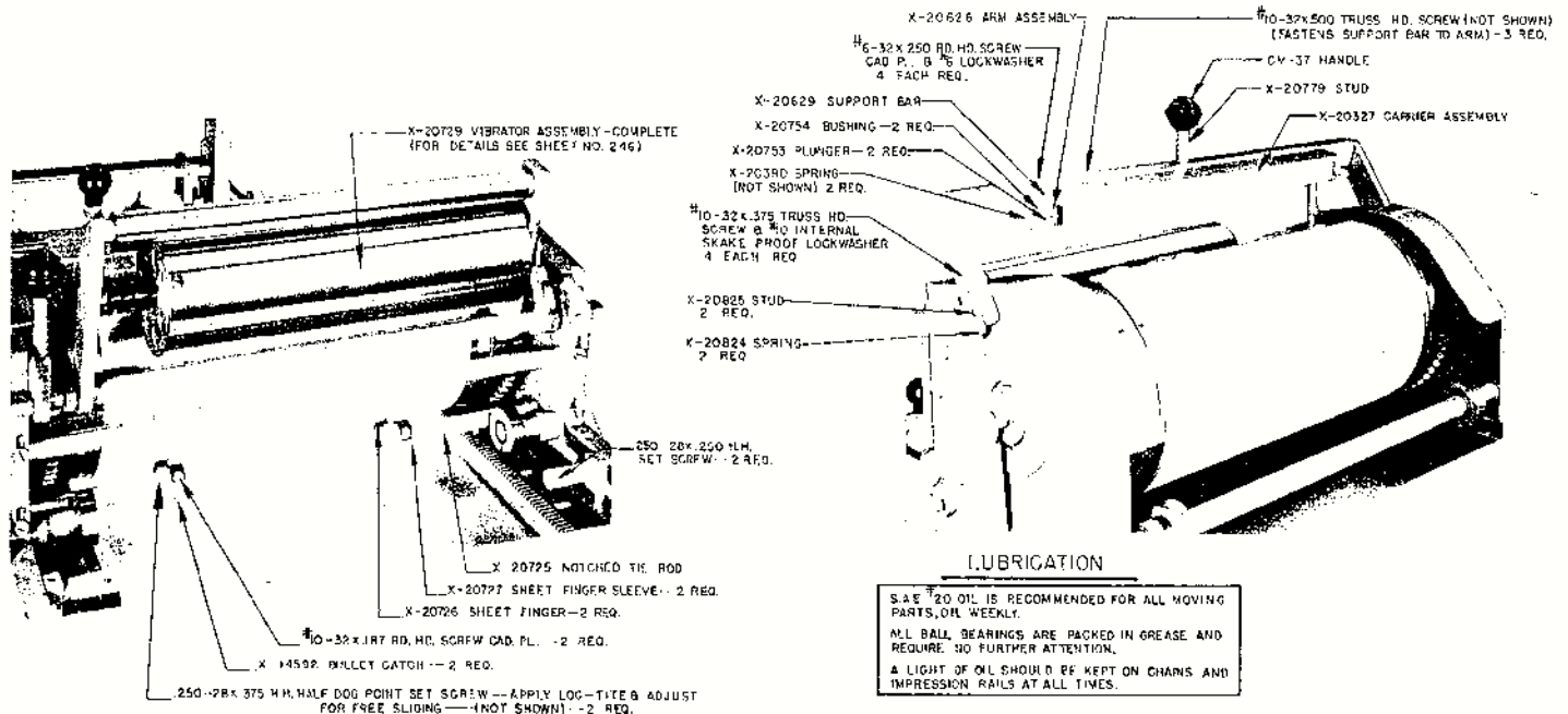
INSIDE VIEW OF CARRIAGE SIDE PLATE—LEFT SIDE
