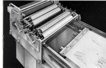
Inking and dampening system—plate clamp.
