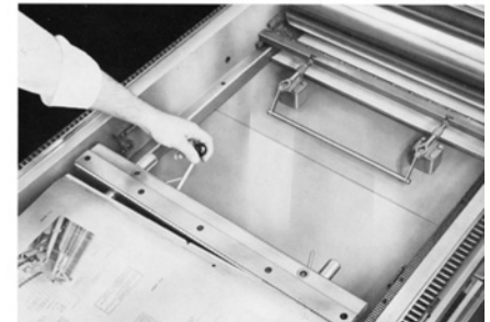
Quick acting plate clamp (not necessary to bend plate)—doctor blade for automatic washup.
