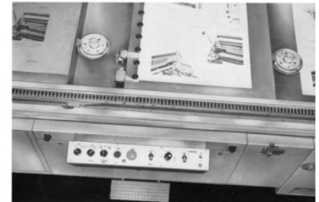
Control panel—gripper pedal—bed height adjusting wheels (no compensating adjustments required)—grippers and micrometer sheet guides.
